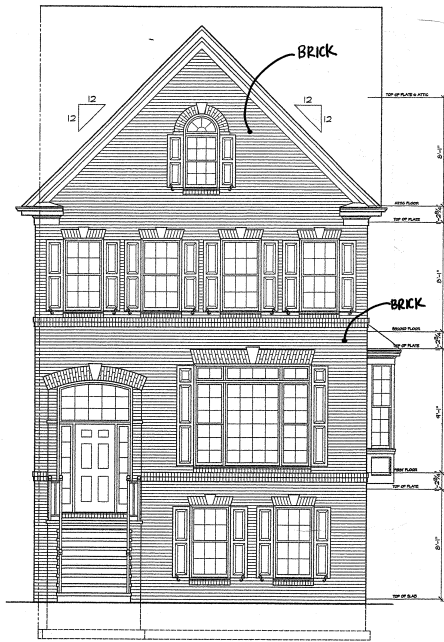
FRONT ELEVATION 1 SLAB-ON-GRADE CONDITION SCALE: 3/4" = 1'-0" (SEE PLAN)
