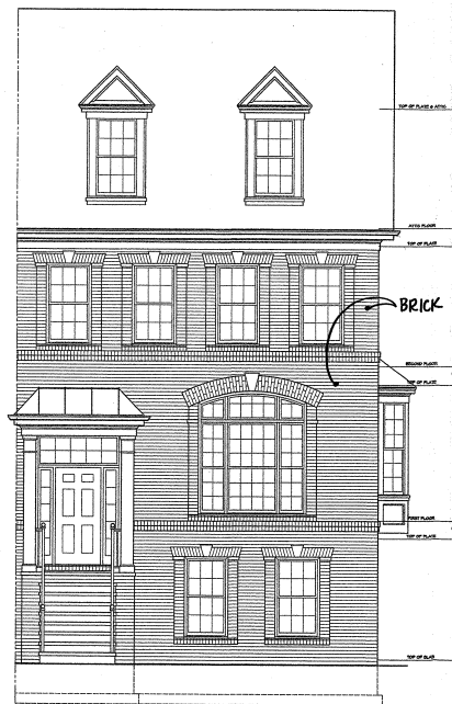
FRONT ELEVATION 3 SLAB-ON-GRADE CONDITION SCALE: 3/4" = 1'-0" (SEE PLAN)
