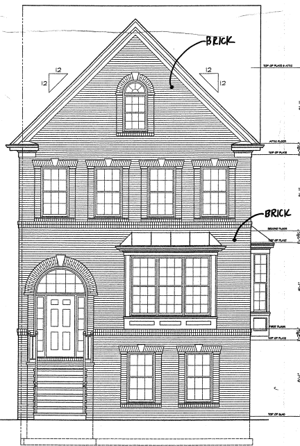
FRONT ELEVATION 2 SLAB-ON-GRADE CONDITION SCALE: 3/4" = 1'-0" (SEE PLAN)
