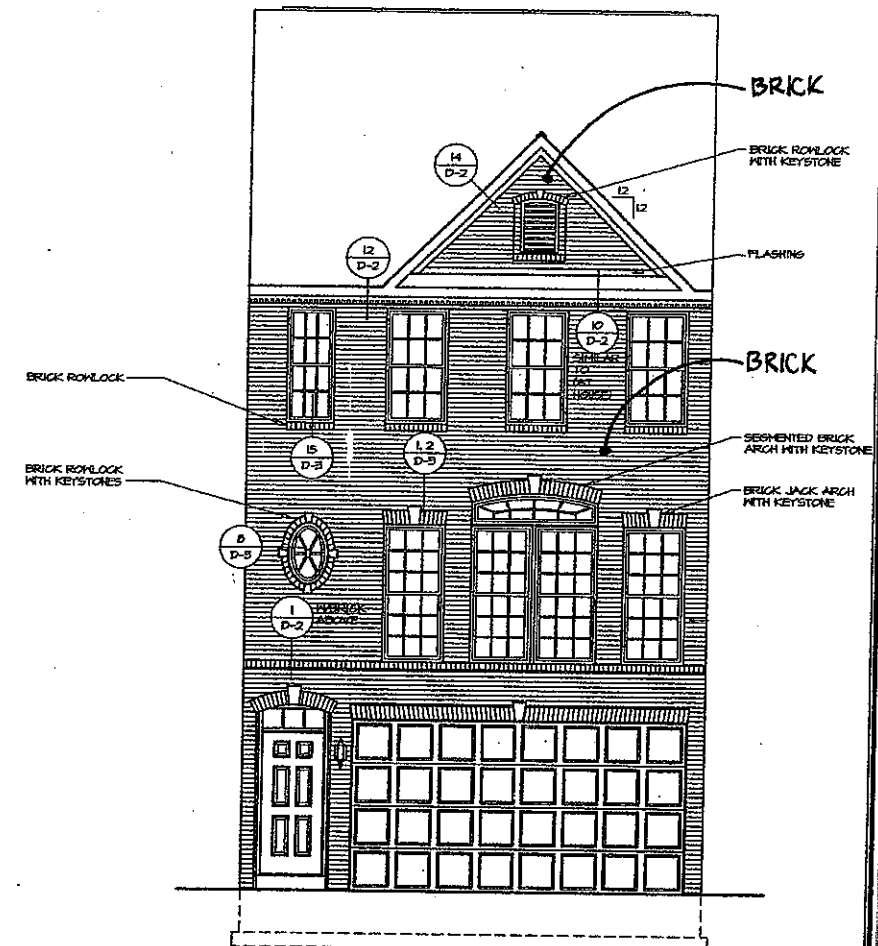
2 FRONT ELEVATION "D" SCALE: 1/4" = 1'-0"
