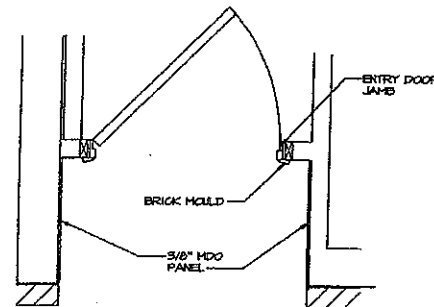
6 ENTRY DOOR TRIM DETAIL SCALE: 3/4" = 1'-0"
