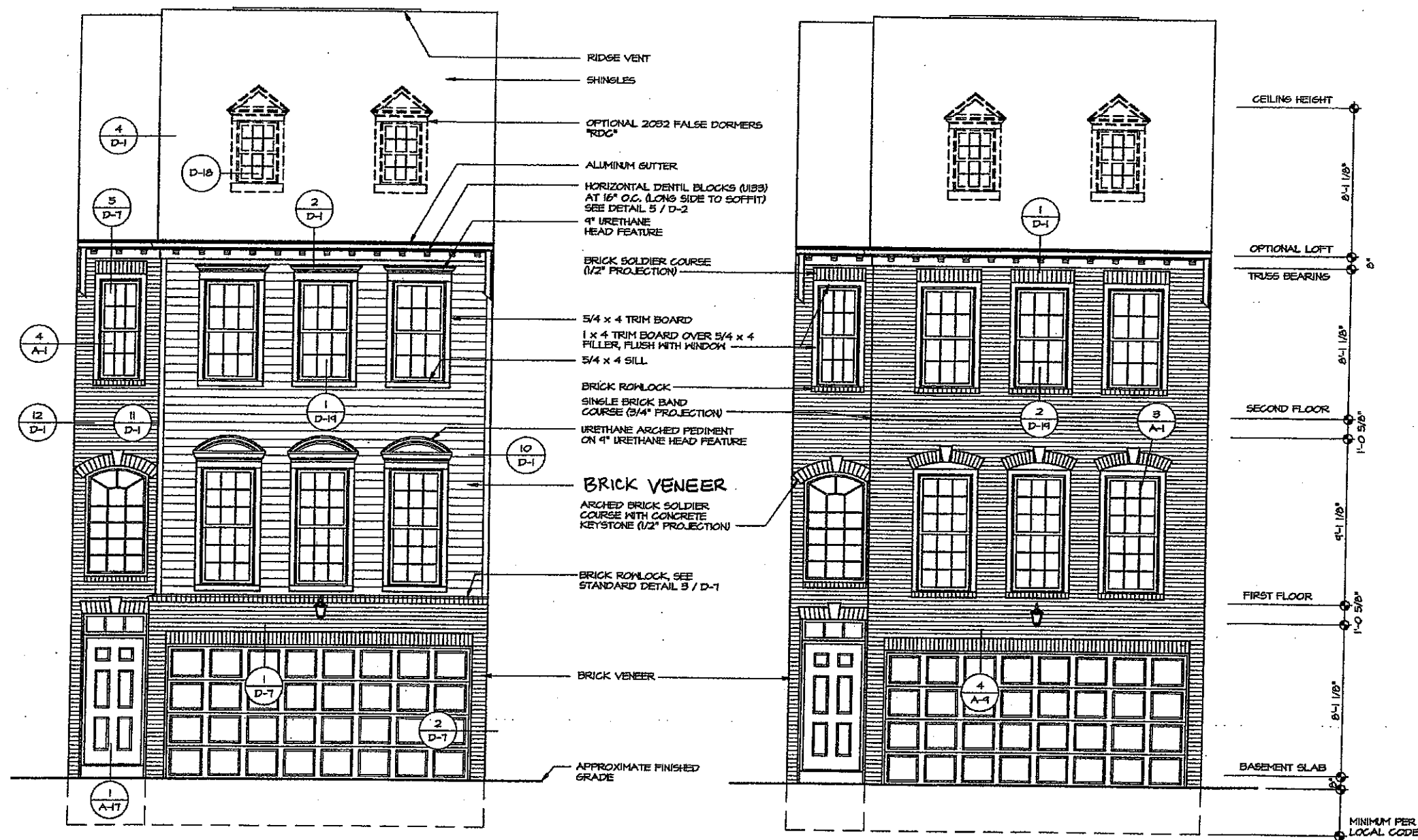
1 FRONT ELEVATION w/ PARTIAL BRICK SCALE: 1/4" = 1'-0" EVA
