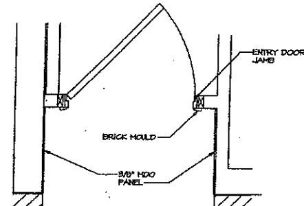
6 ENTRY DOOR TRIM DETAIL SCALE: 3/4" = 1'-0"
