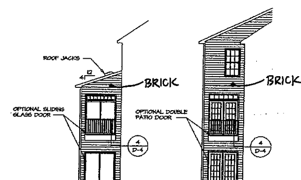
15 LEFT SIDE ELEVATION SCALE 1/8" = 1'-0" WALKOUT WITH REAR SUNROOM "MAY" WITHOUT LUXURY OWNER'S SUITE
