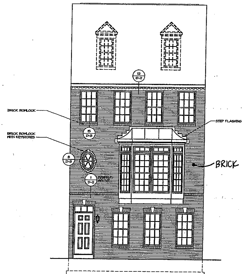
2 FRONT ELEVATION "E" SCALE: 1/4" = 1'-0"
