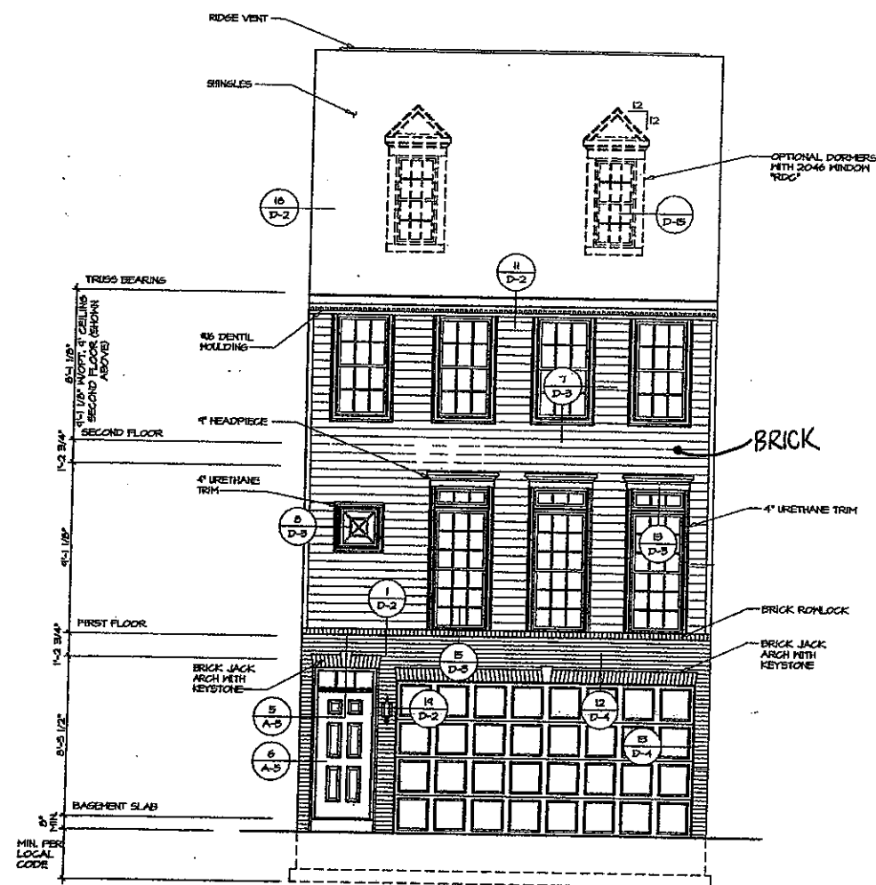
1 FRONT ELEVATION "A" SCALE: 1/4" = 1'-0"
