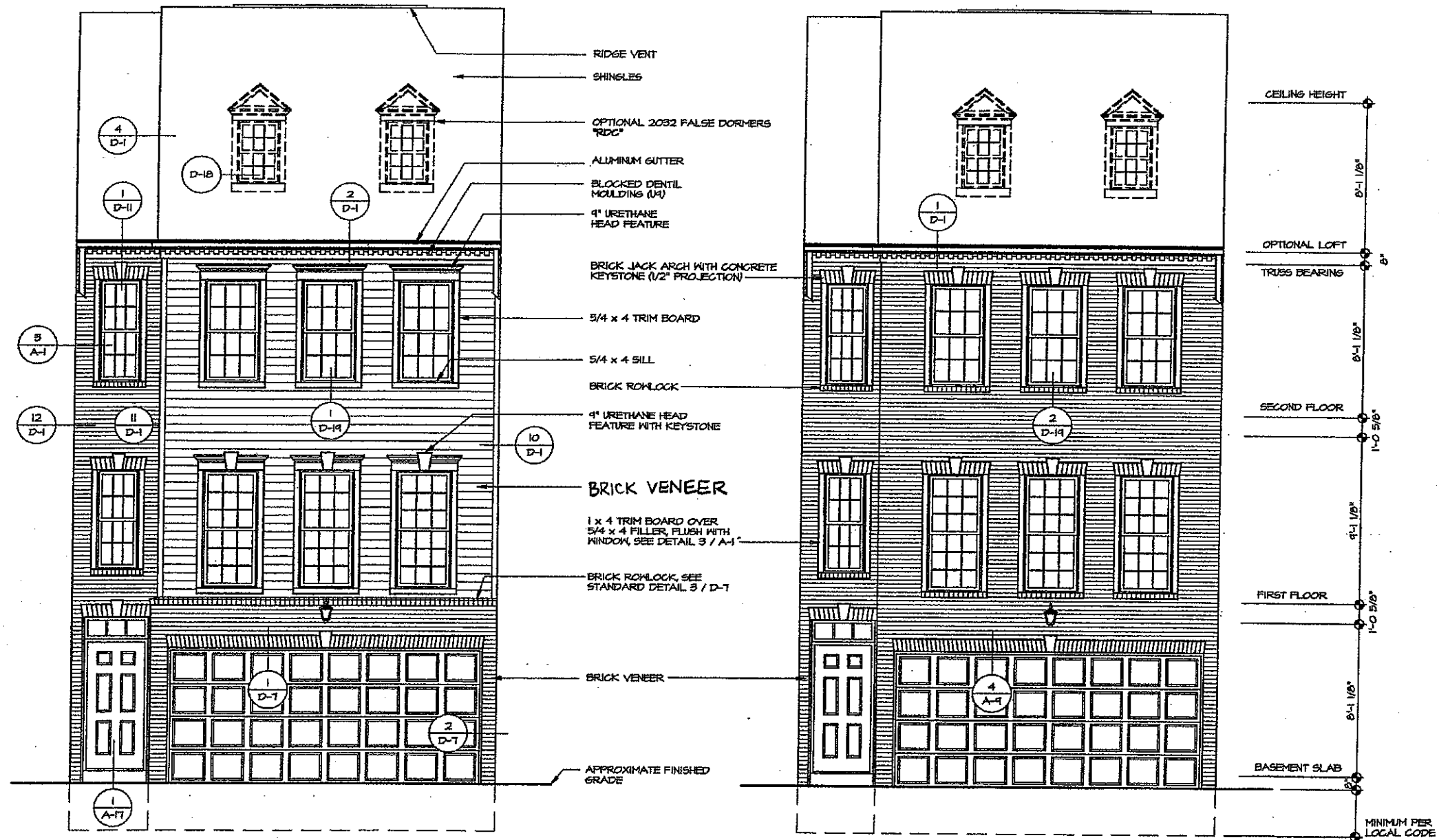
1 A-1 FRONT ELEVATION w/ PARTIAL BRICK SCALE: 1/4" = 1'-0" "EVA"
