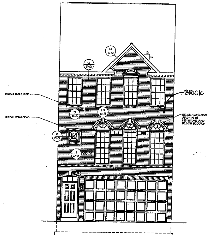
2 FRONT ELEVATION "C" SCALE: 1/4" = 1'-0"
