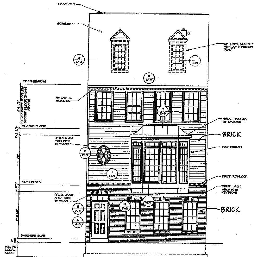
1 FRONT ELEVATION "E" SCALE: 1/4" = 1'-0"
