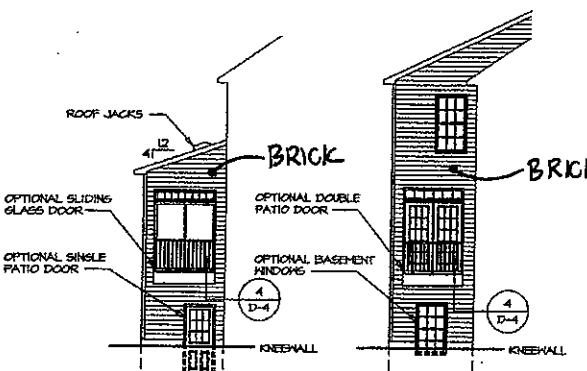
13 LEFT SIDE ELEVATION SCALE 1/8" = 1'-0" KNEEWALL WITH REAR SUNROOM "MAY" WITHOUT LUXURY OWNER'S SUITE
