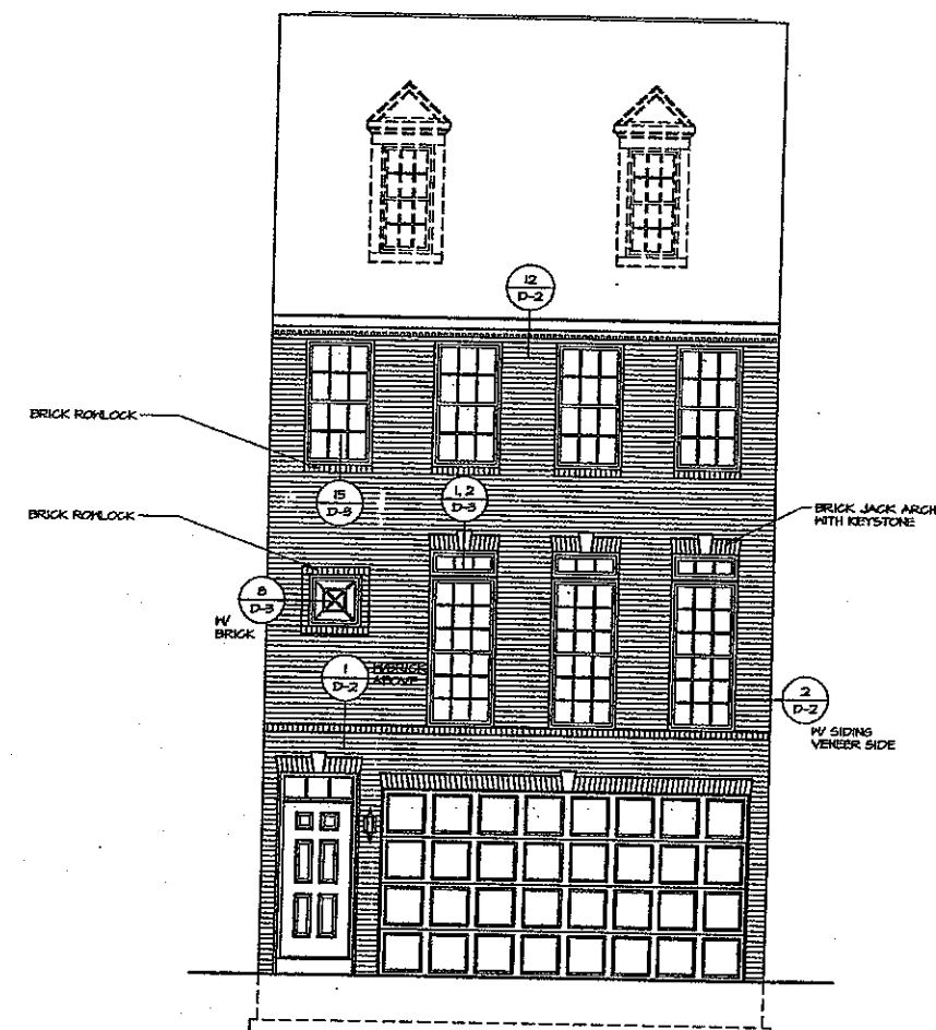
2 FRONT ELEVATION "A" SCALE: 1/4" = 1'-0"
