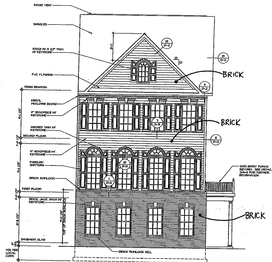
2 FRONT ELEVATION "B" SCALE 1/4" = 1'-0" BASEMENT LEVEL, ENTRY/GARAGE "TIE" SIDE ENTRY "ETB"
