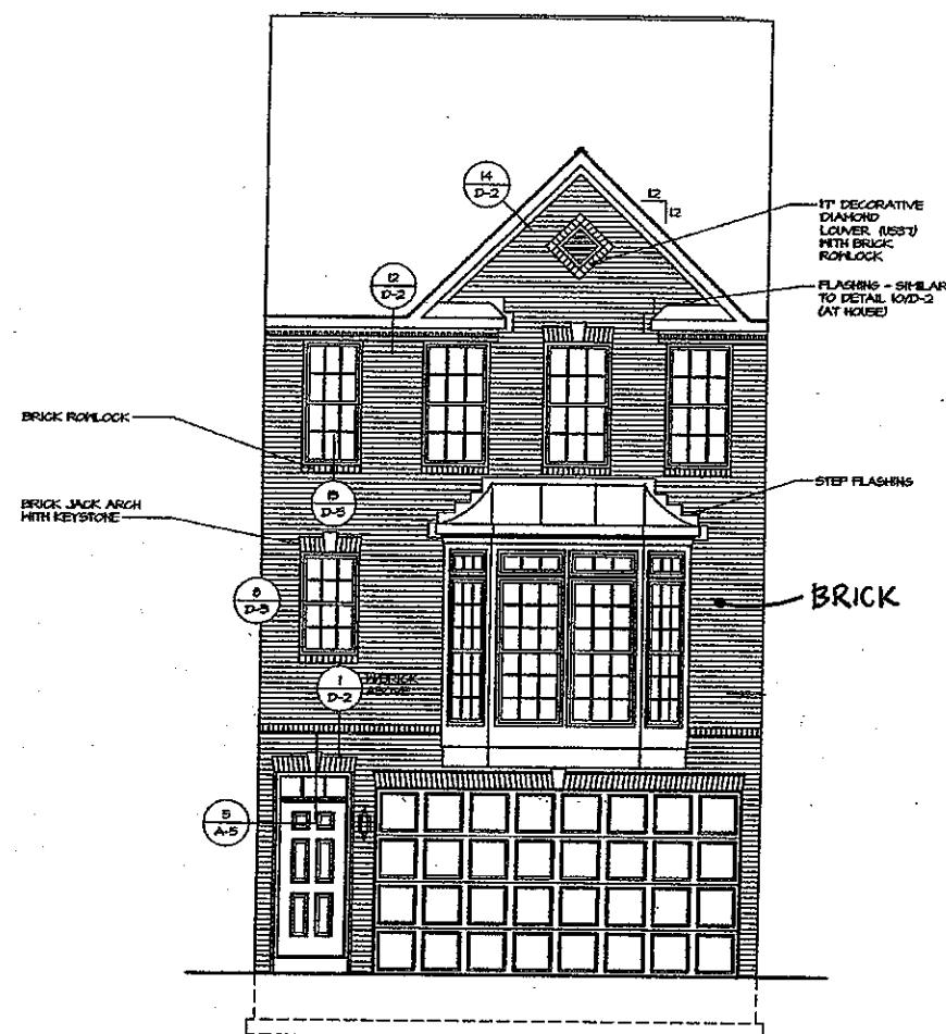
2 FRONT ELEVATION "F" SCALE: 1/4" = 1'-0" BRICK VENEER FRONT "EVA" 14" OPT. 4" CEILING SECOND FLOOR "SC"
