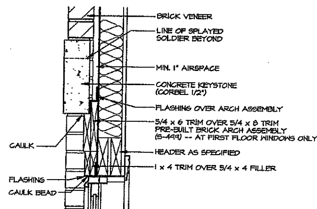
3 HEADPIECE SECTION SCALE: 1/4" = 1'-0"
