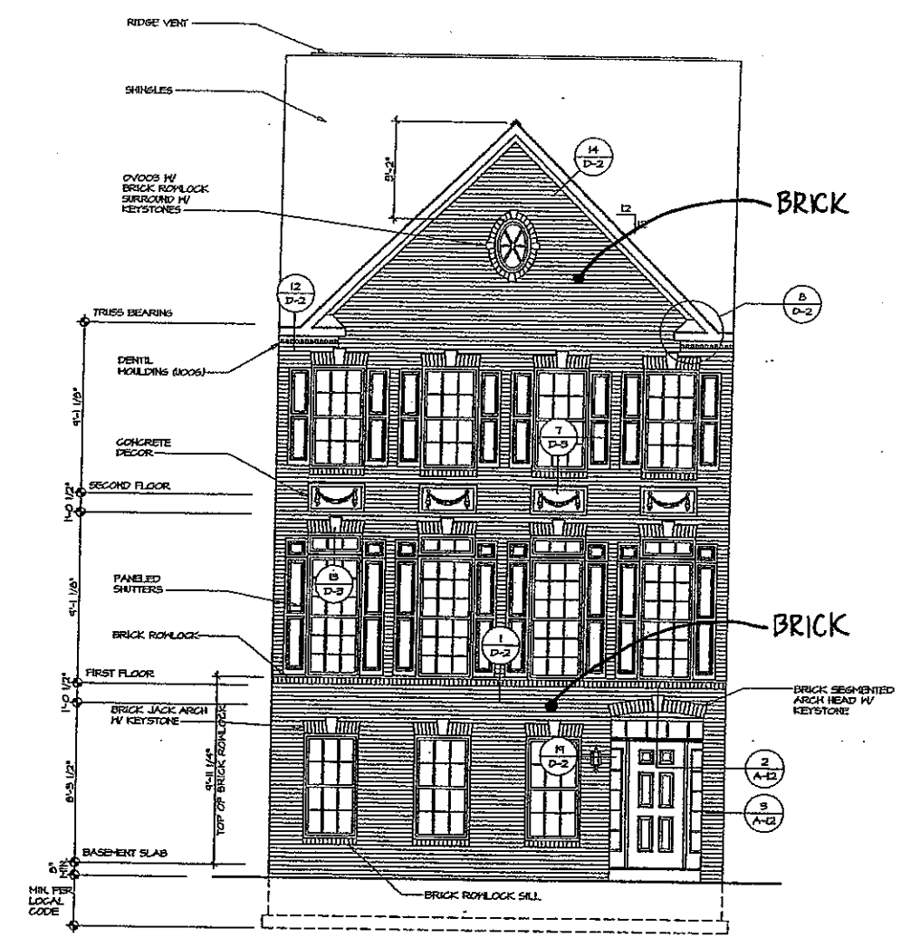
2 FRONT ELEVATION "F" SCALE 1/4" = 1'-0" BASEMENT LEVEL ENTRY "FIE" FRONT ENTRY "EIA"
