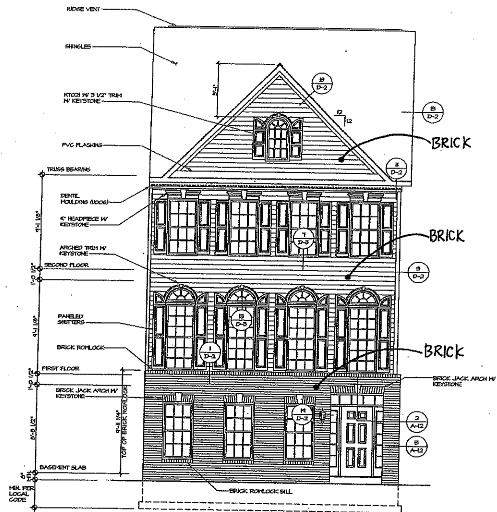
1 FRONT ELEVATION "B" SCALE 1/4" = 1'-0" BASEMENT ENTRY W/ GARAGE "TIE" FRONT ENTRY "EIA"
