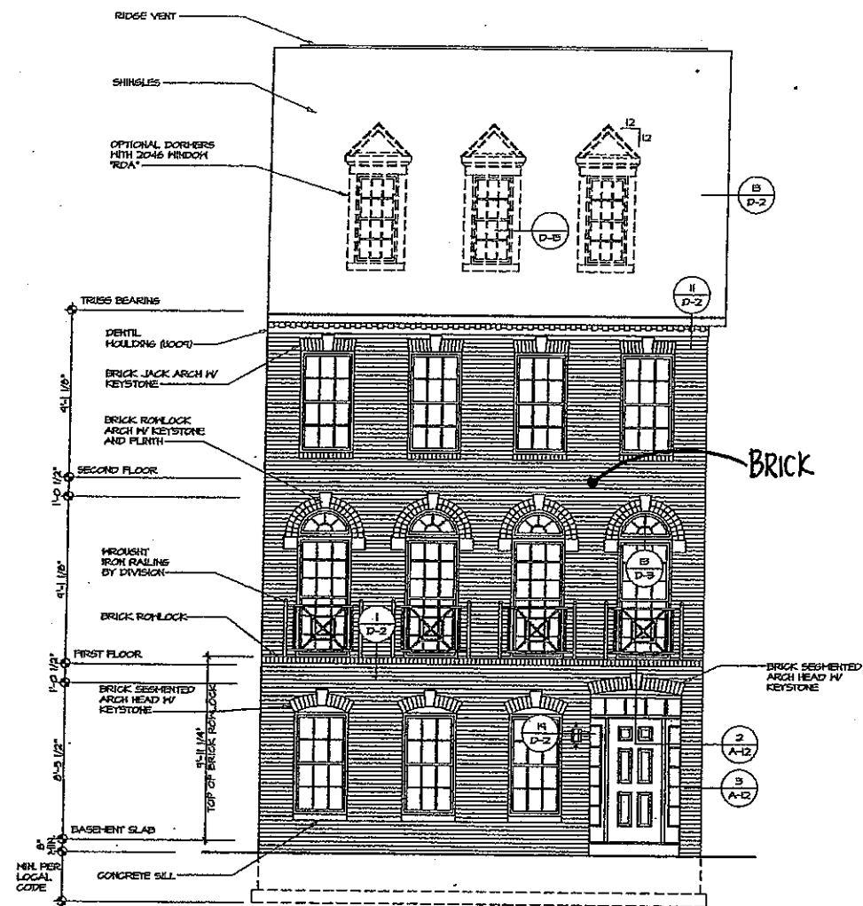
1 FRONT ELEVATION "D" SCALE 1/4" = 1'-0" BASEMENT LEVEL ENTRY "FIE" FRONT ENTRY "E1A"
