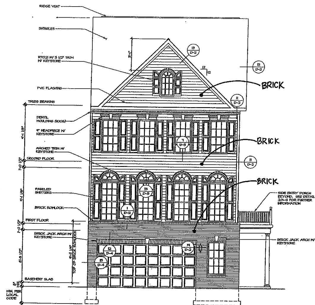
2 FRONT ELEVATION "B" SCALE: 1/4" = 1'-0" BASEMENT LEVEL ENTRY W/ GARAGE "F1D" SIDE ENTRY "E1B"
