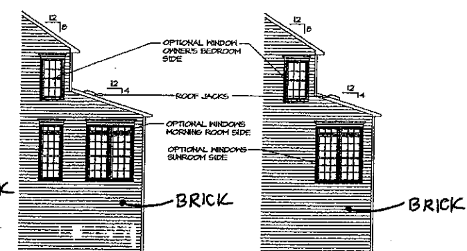
9 RIGHT SIDE ELEVATION SCALE 1/8" = 1'-0" WALKOUT WITH MORNING ROOM "MAY" WITHOUT LUXURY OWNER'S SUITE
