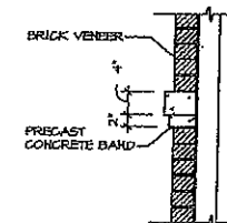
3 PRECAST CONCRETE BAND DETAIL SCALE 3/4" = 1'-0"
