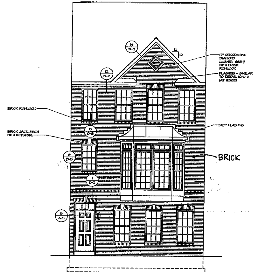
2 FRONT ELEVATION "F" SCALE: 1/4" = 1'-0" BRICK VENEER FRONT "EVN" W/ 8" CEILING SECOND FLOOR "SCF"
