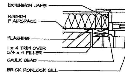
3 WINDOW TRIM SECTION SCALE: 1 1/2\"/>
