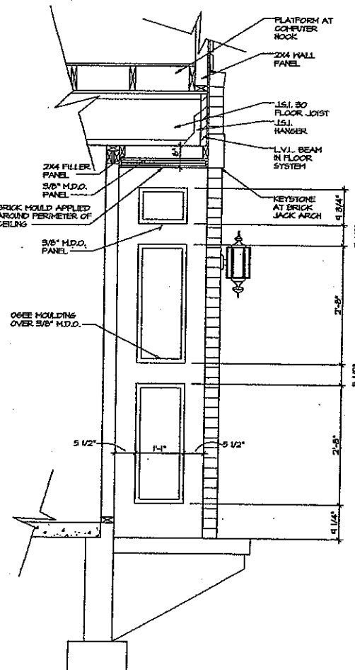
5 RECESSED ENTRY DETAIL SCALE: 3/4" = 1'-0"
