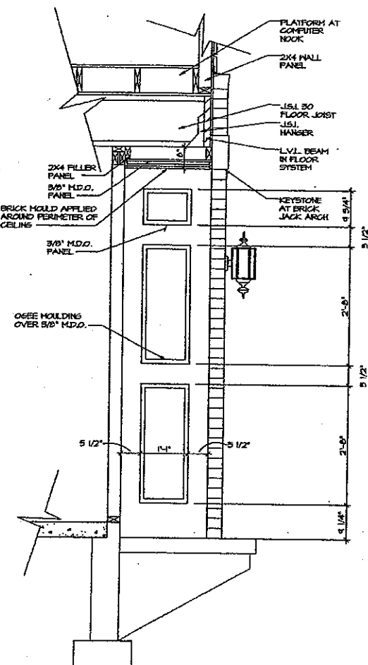
5 RECESSED ENTRY DETAIL SCALE: 3/4" = 1'-0"
