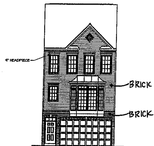
9 FRONT ELEVATION "F" SCALE: 1/8" = 1'-0" BRICK VENEER FRONT "EVA" 14" OPT. 4" CEILING SECOND FLOOR "SC"
