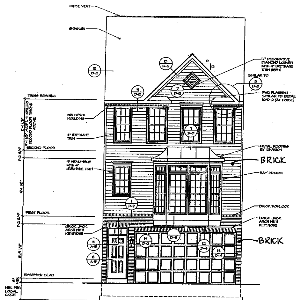
1 FRONT ELEVATION "F" SCALE: 1/4" = 1'-0" BRICK VENEER FRONT "EVA" 14" OPT. 4" CEILING SECOND FLOOR "SC"
