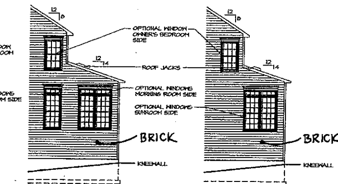
7 RIGHT SIDE ELEVATION SCALE 1/8" = 1'-0" KNEEWALL WITH MORNING ROOM "MAY" WITHOUT LUXURY OWNER'S SUITE
