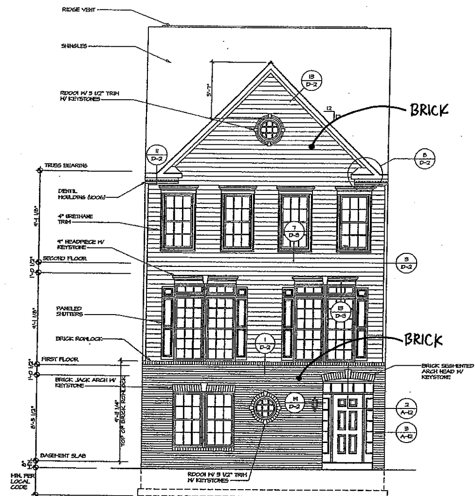
2 FRONT ELEVATION "C" A-5 SCALE 1/4" = 1'-0" BASEMENT LEVEL ENTRY "FTE" FRONT ENTRY "ETA"
