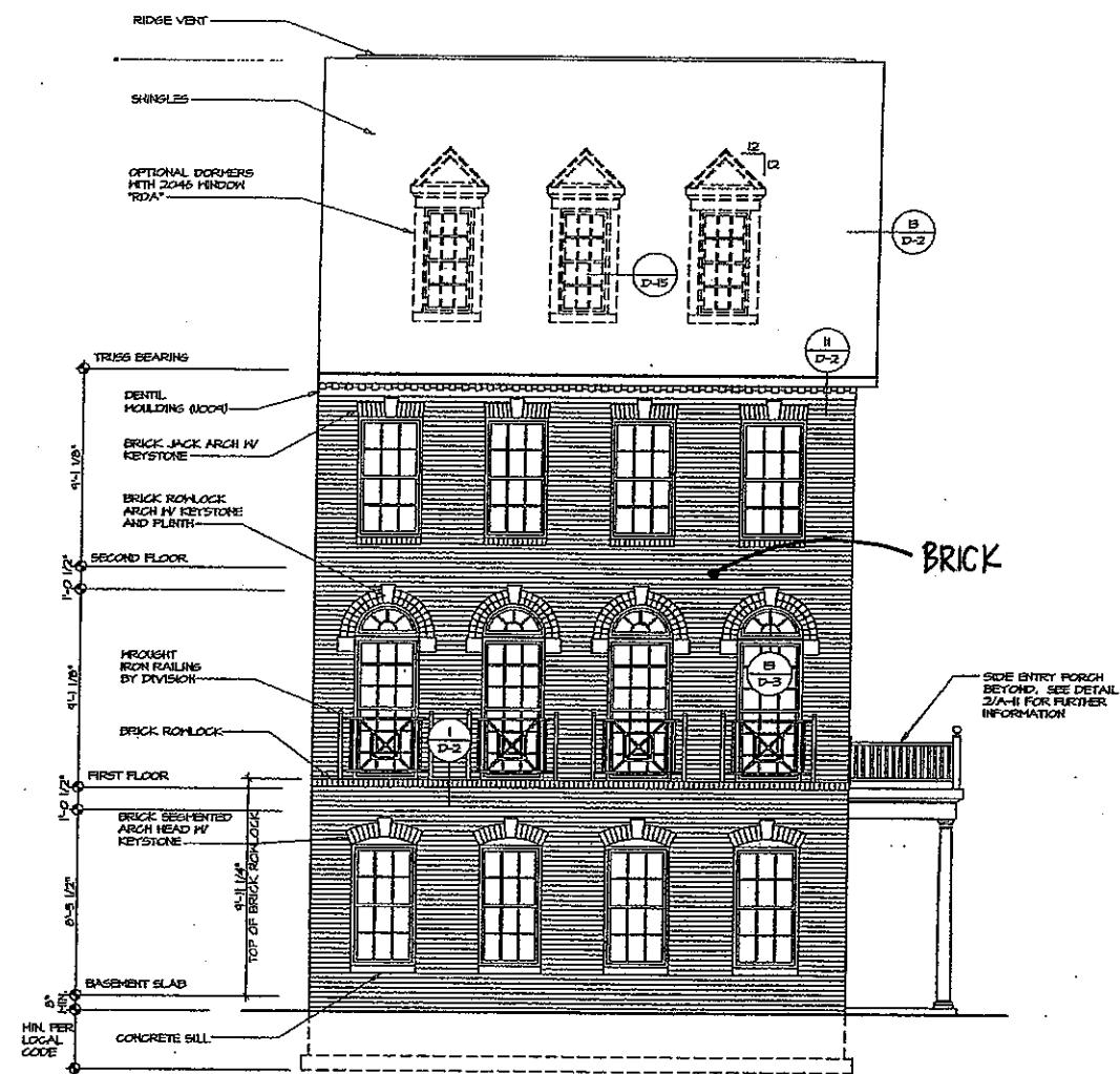
2 FRONT ELEVATION "D" SCALE 1/4" = 1'-0" BASEMENT LEVEL ENTRY "FIE" SIDE ENTRY "E1B"
