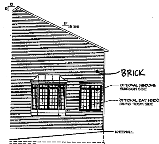
11 RIGHT SIDE ELEVATION SCALE 1/8" = 1'-0" KNEEWALL WITH REAR SUNROOM AND LUXURY OWNER'S SUITE "MAY" AND "LBY"
