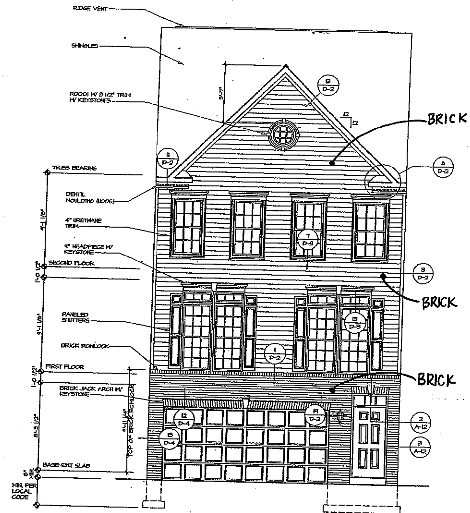
2 FRONT ELEVATION "C" SCALE: 1/4" = 1'-0" BASEMENT LEVEL ENTRY W/ GARAGE "TID" FRONT ENTRY "ETA"
