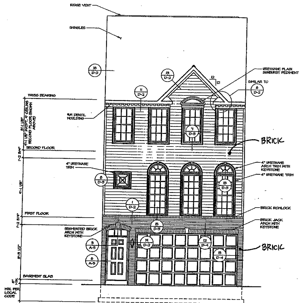
1 FRONT ELEVATION "C" SCALE: 1/4" = 1'-0"
