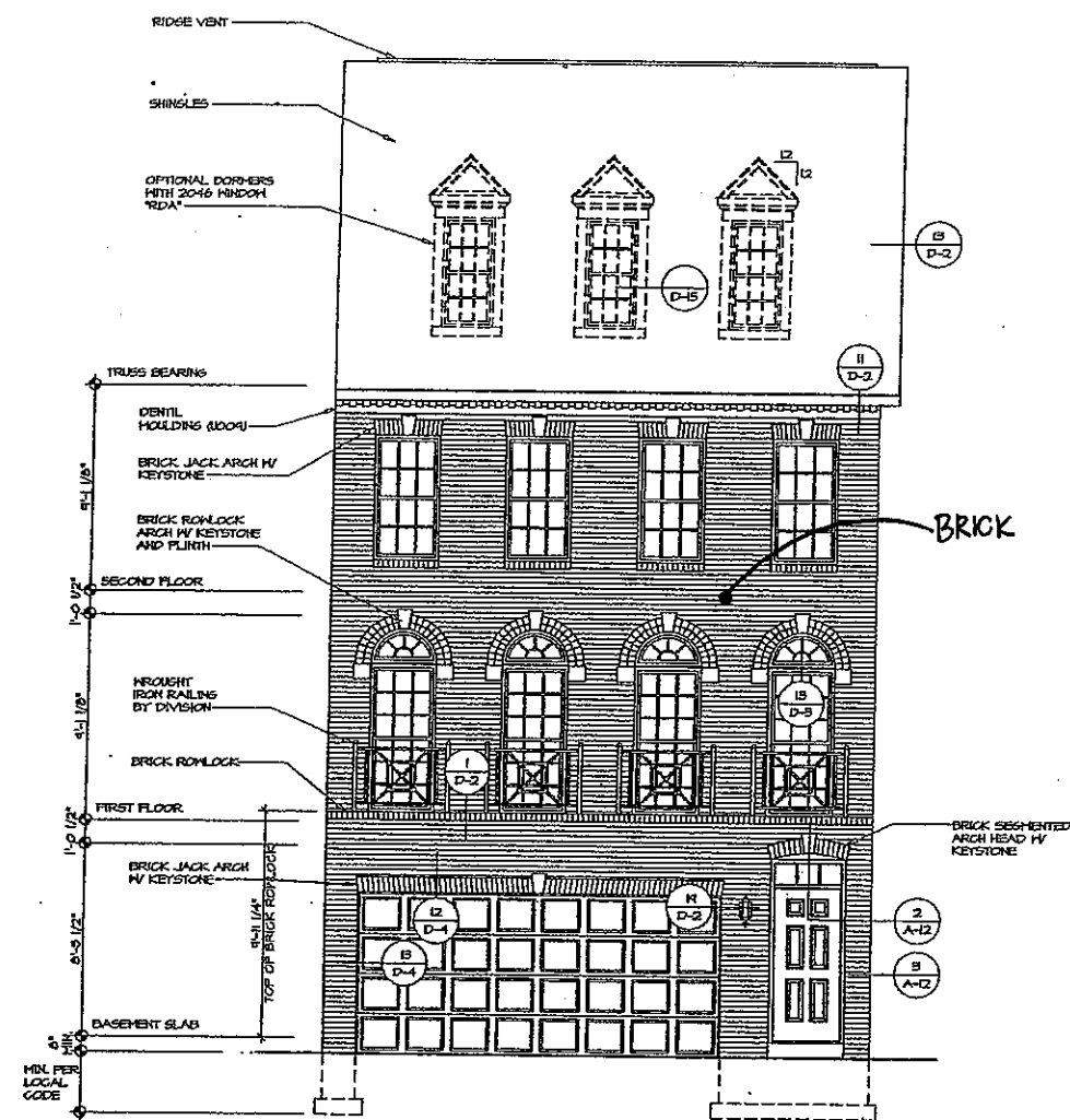
1 FRONT ELEVATION "D" SCALE: 1/4" = 1'-0" BASEMENT LEVEL ENTRY IN GARAGE "ETD" FRONT ENTRY "ETB"
