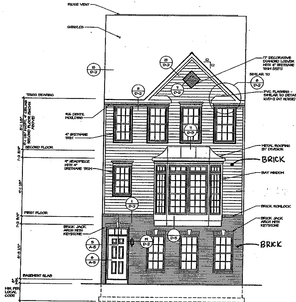
1 FRONT ELEVATION "F" SCALE: 1/4" = 1'-0" BRICK VENEER FRONT "EVN" W/ 8" CEILING SECOND FLOOR "SCF"
