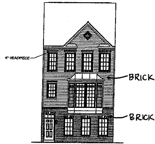
3 FRONT ELEVATION "F" SCALE: 1/8" = 1'-0" BRICK VENEER FRONT "EVN" W/ OPT. 4" CEILING SECOND FLOOR "SCF"
