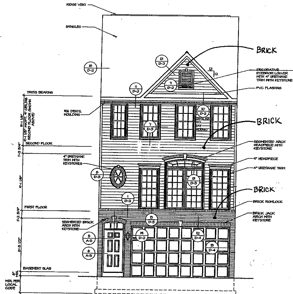
1 FRONT ELEVATION "D" SCALE: 1/4" = 1'-0"
