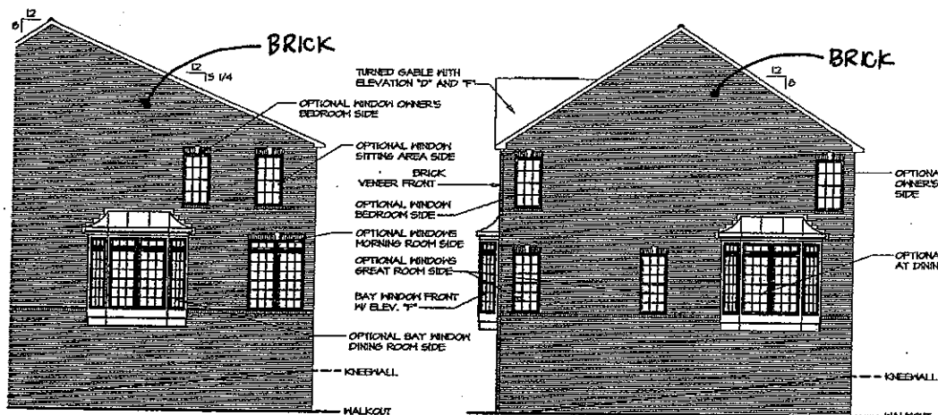
5 RIGHT SIDE ELEVATION SCALE 1/8" = 1'-0" WALKOUT WITH MORNING RM. AND LUXURY OWNER'S SUITE "MAY" AND "LBY"
