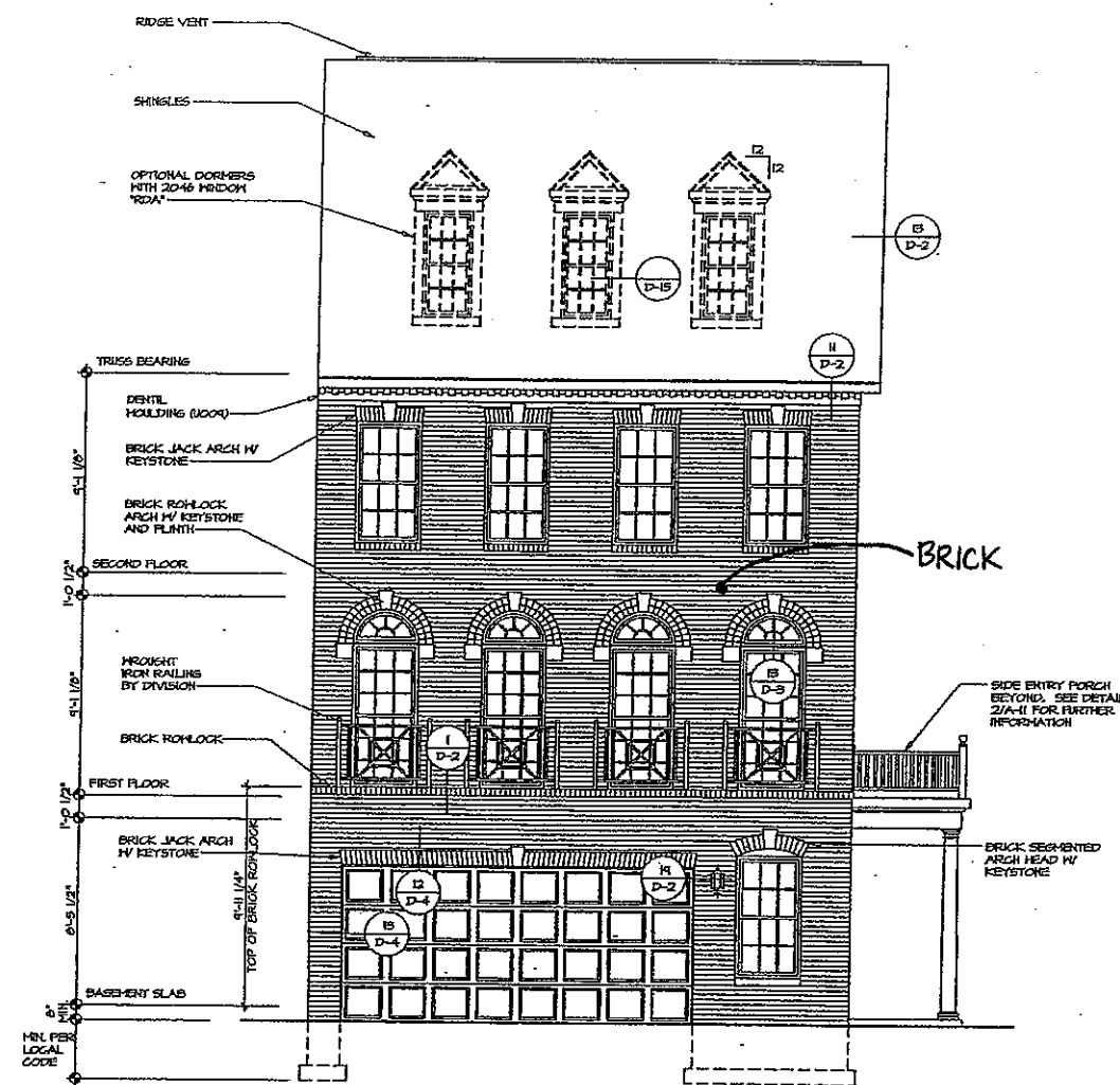
2 FRONT ELEVATION "D" SCALE: 1/4" = 1'-0" BASEMENT LEVEL ENTRY IN GARAGE "ETD" SIDE ENTRY "ETB"
