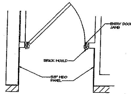
6 ENTRY DOOR TRIM DETAIL SCALE: 3/4" = 1'-0"
