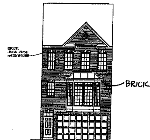
4 FRONT ELEVATION "F" SCALE: 1/8" = 1'-0" BRICK VENEER FRONT "EVA" 14" OPT. 4" CEILING SECOND FLOOR "SC"
