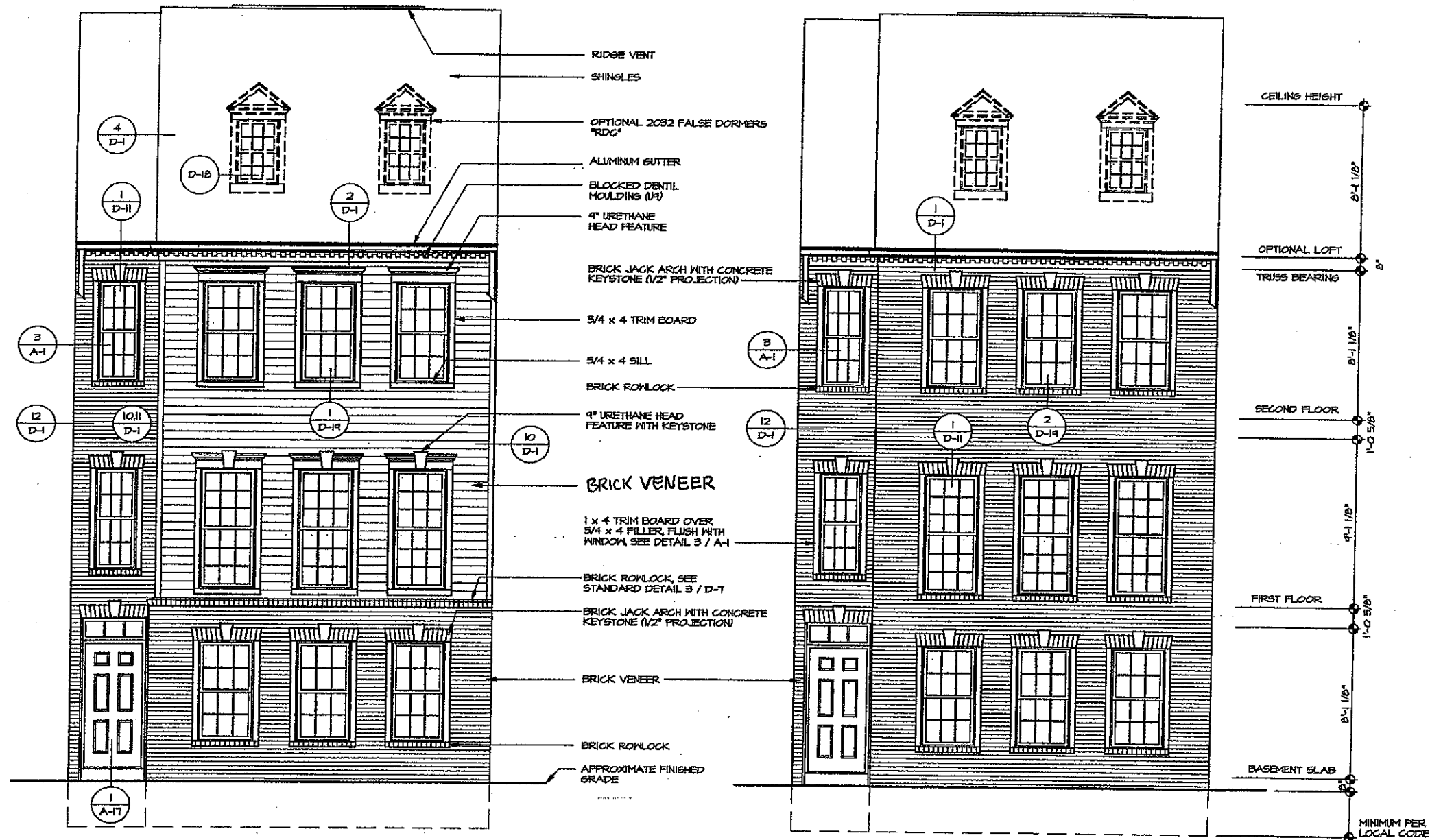
1 FRONT ELEVATION W/ PARTIAL BRICK SCALE: 1/4\"/>
