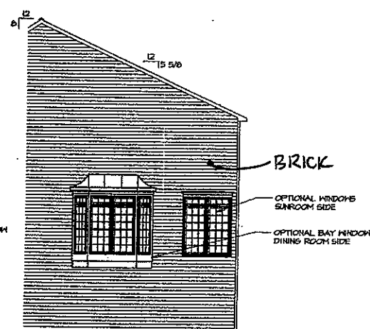
12 RIGHT SIDE ELEVATION SCALE 1/8" = 1'-0" WALKOUT WITH REAR SUNROOM AND LUXURY OWNER'S SUITE "MAY" AND "LBY"
