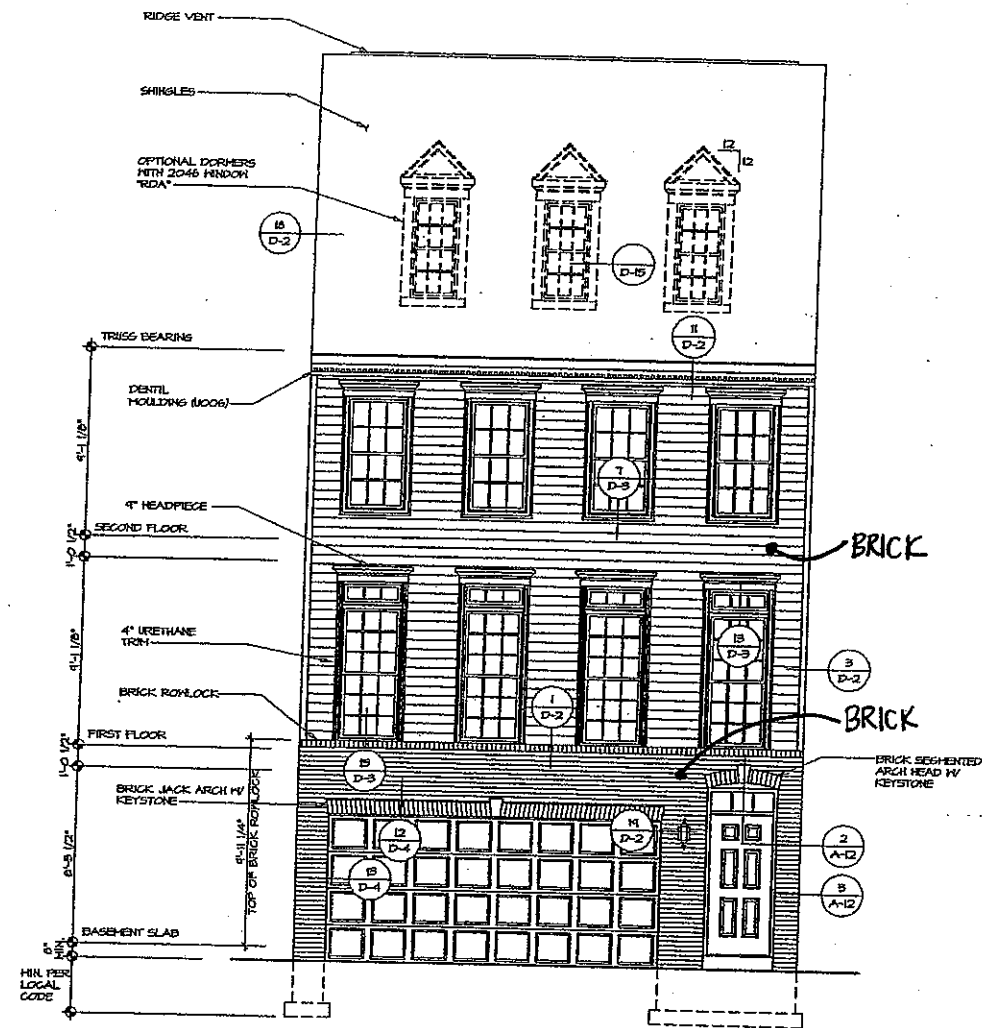
1 FRONT ELEVATION "A" SCALE: 1/4" = 1'-0" BASEMENT LEVEL ENTRY W/ GARAGE "TID" FRONT ENTRY "ETA"
