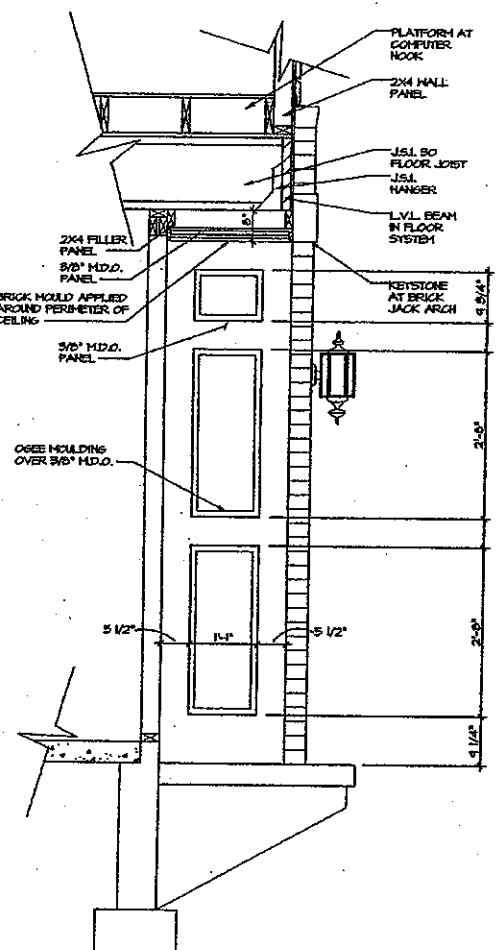
5 RECESSED ENTRY DETAIL SCALE: 5/8" = 1'-0"
