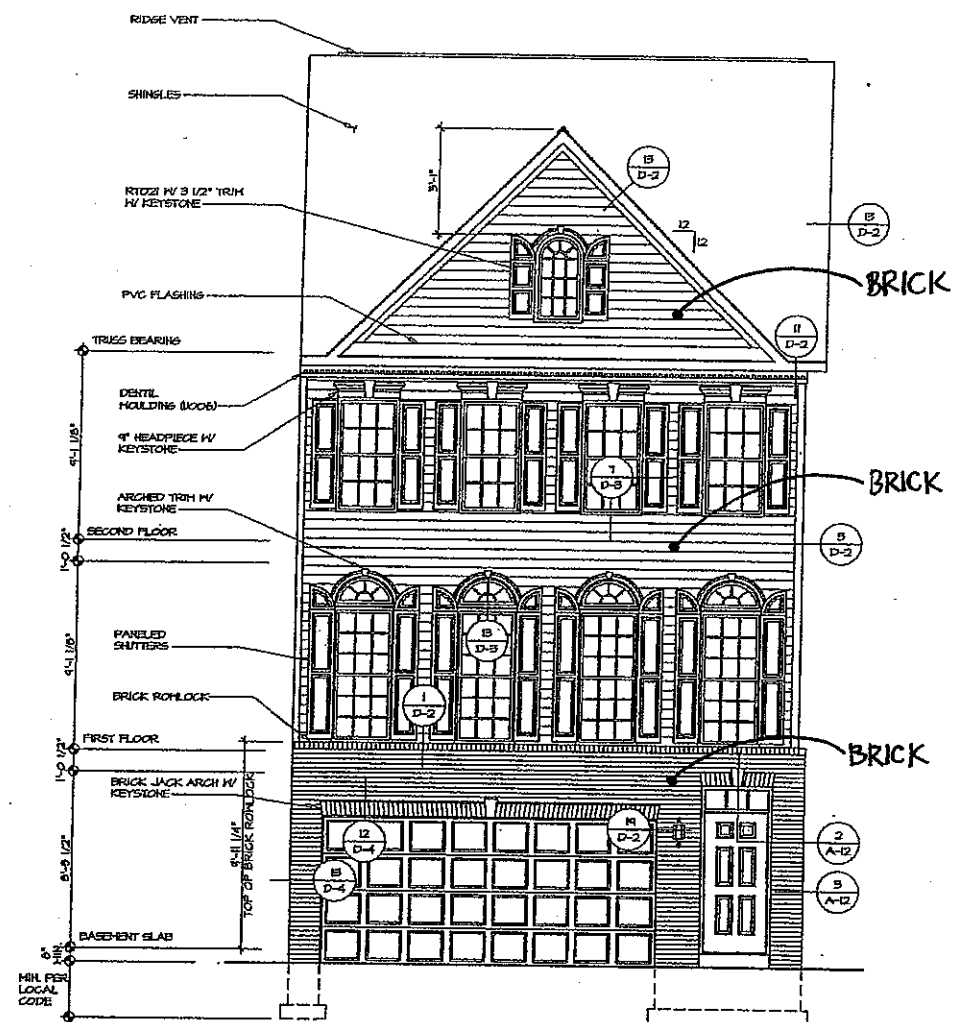
1 FRONT ELEVATION "B" SCALE: 1/4" = 1'-0" BASEMENT LEVEL ENTRY W/ GARAGE "F1D" FRONT ENTRY "E1A"
