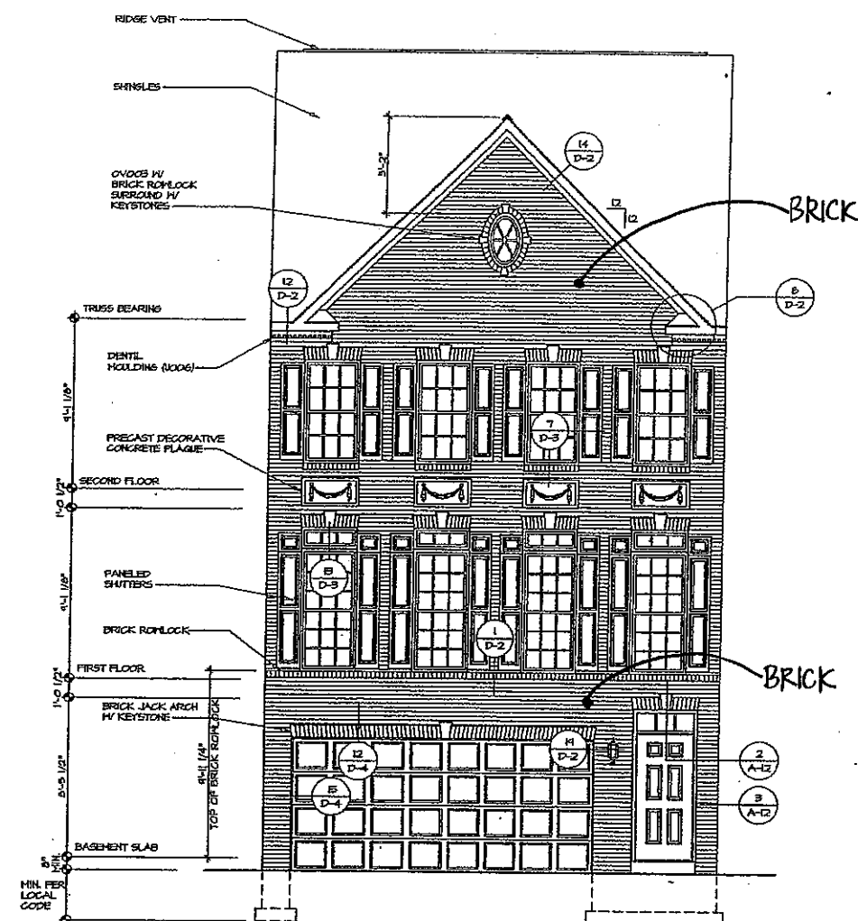
BASMENT LEVEL ENTRY W/ GARAGE "FD" FRONT ENTRY "ETA"
