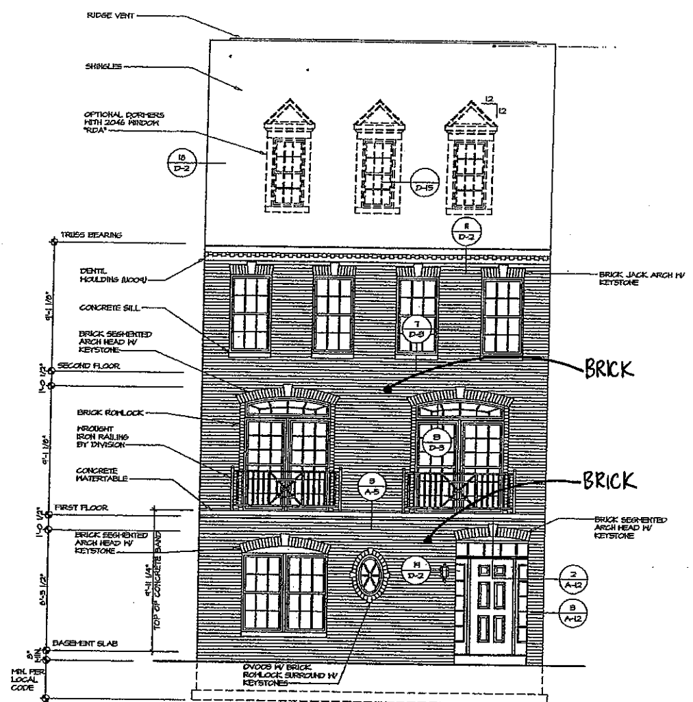
1 FRONT ELEVATION "E" SCALE 1/4" = 1'-0" BASEMENT LEVEL ENTRY "FIE" FRONT ENTRY "EIA"
