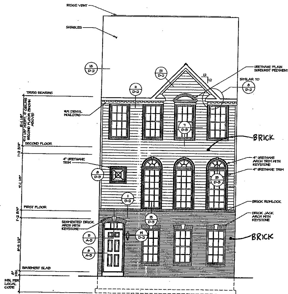
1 FRONT ELEVATION "C" SCALE: 1/4" = 1'-0"
