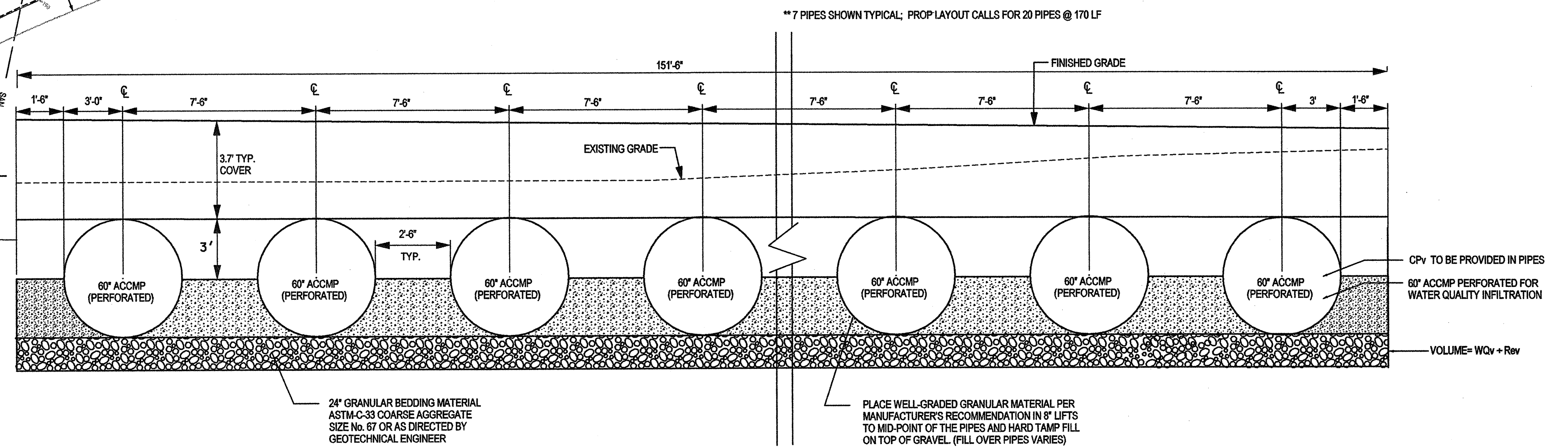
UNDERGROUND SWM FACILITY - SEC. "A-A"
